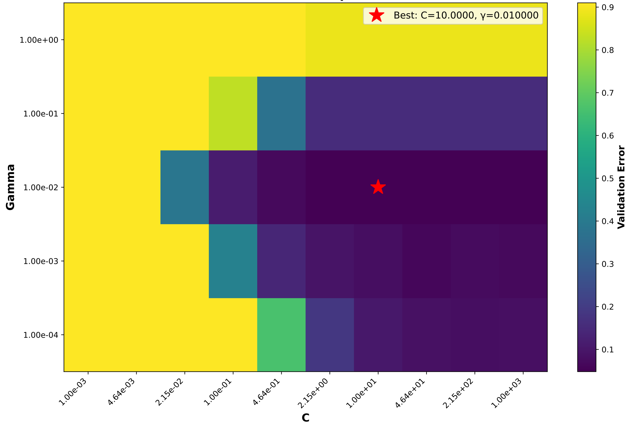
Validation Error Heatmap (RBF Kernel)
